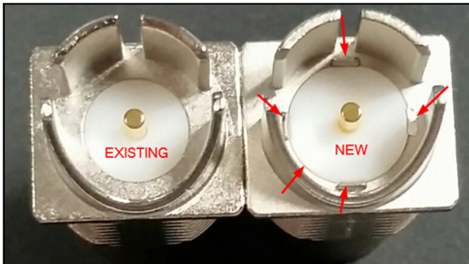
Existing & New Design (Rear View)
