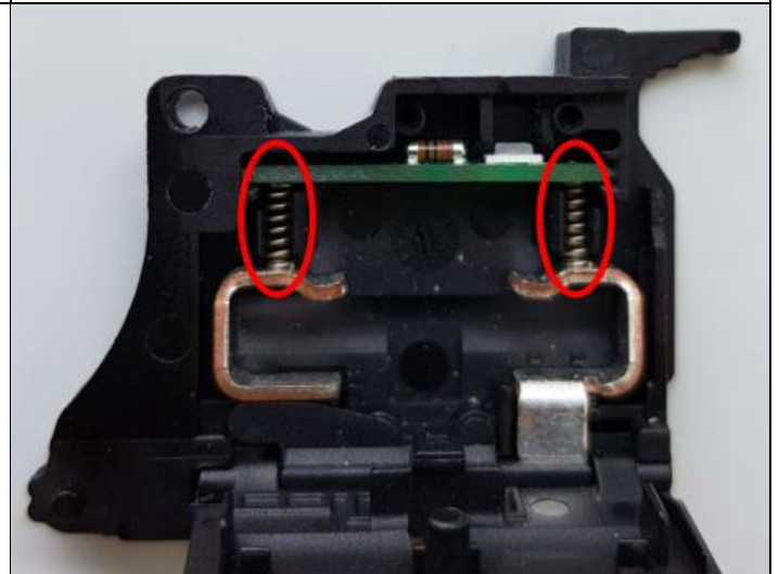
The addition of springs means that the HESI LED levers provide better contact quality.
