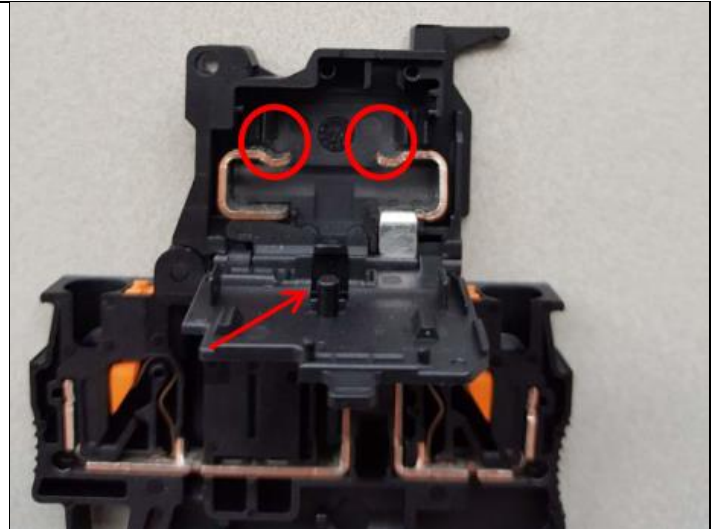
The design of the metal latch was adapted, and the tab to hold the fuse changed.
