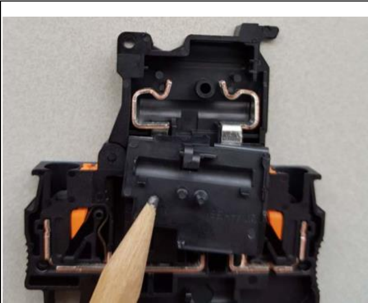
The design of the metal latch was adapted, and the tab to hold the fuse changed.
